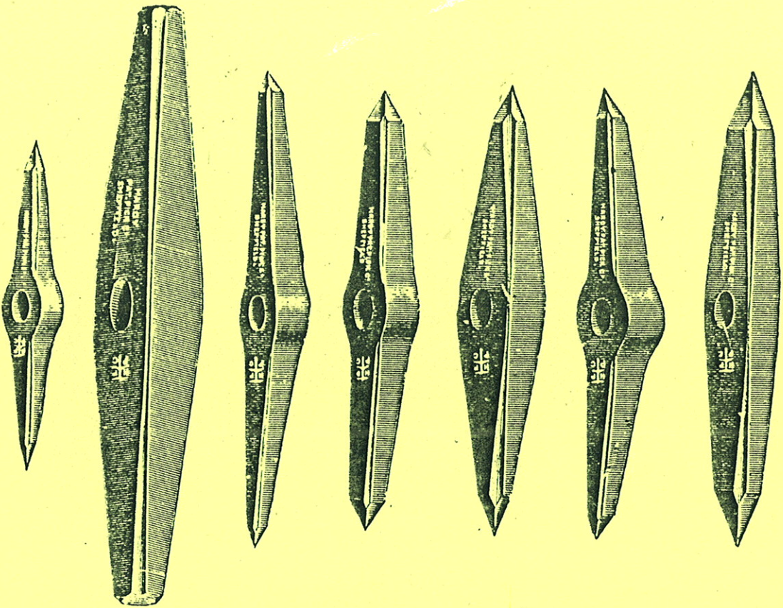
FIG. 163. Quarry picks (Hardy Patent Pick Co., Ltd.).
